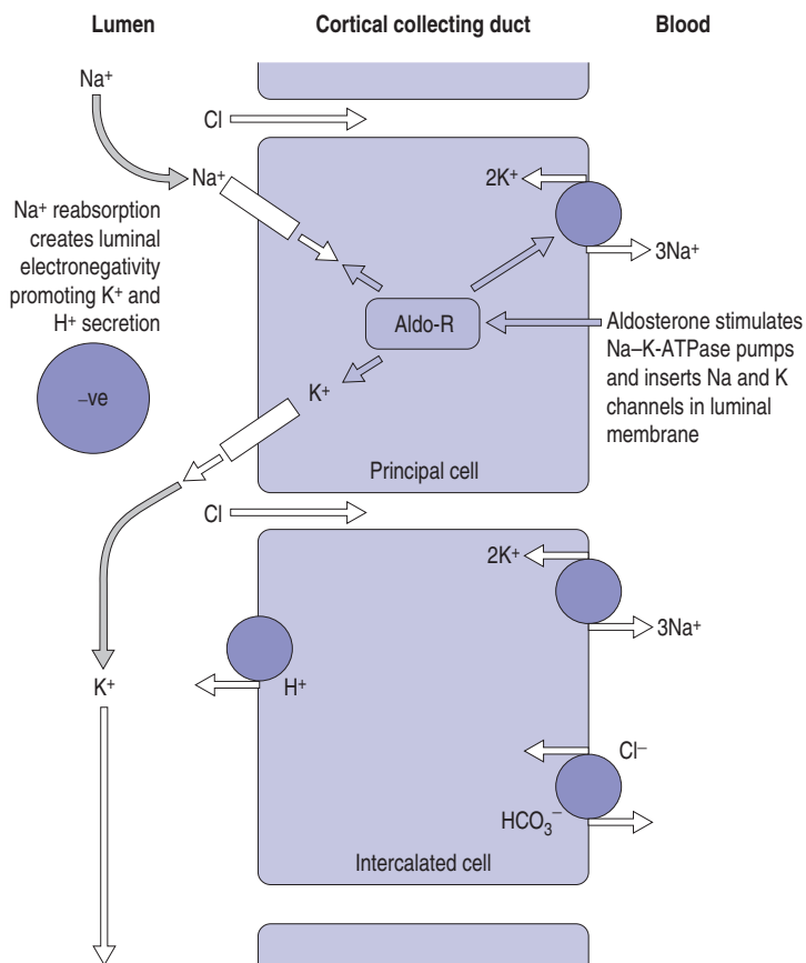
Figure 2.2 Renal excretion of potassium. Potassium secretion is controlled in the cortical collecting duct (CCD). Sodium reabsorption in this segment produces a negative voltage gradient, promoting \text{K}^+ secretion under the actions of aldosterone. Aldo-R, aldosterone receptor.
